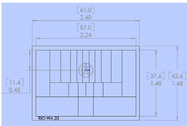
Dimension Schematic WA-23 Lens Array Dimensions: in [mm]
