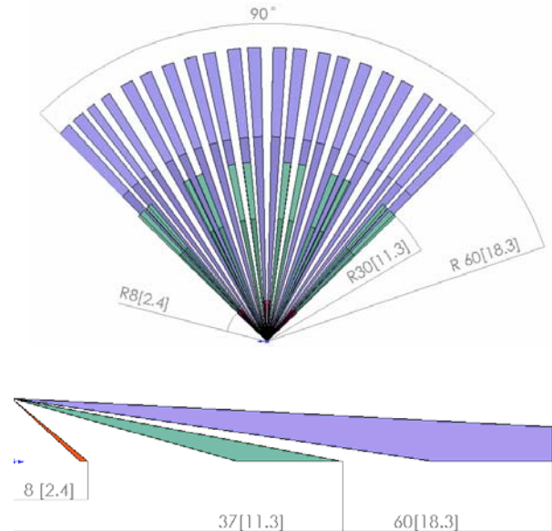
Protection Pattern WA-23 Dimensions: ft. [m]
