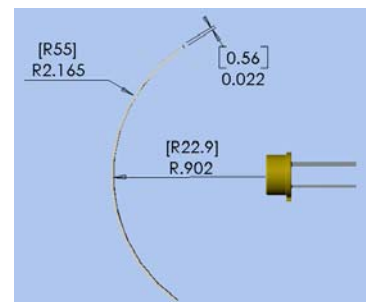
Recommended Installation Dimensions: in [mm]
