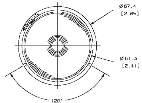
Typical Lens Schematic
