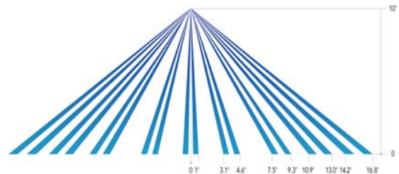
Protection Pattern Dimensions in ft. (m)
